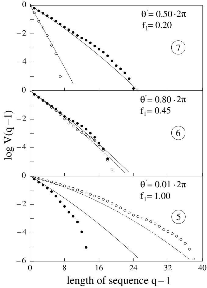
Figure 5. Probability U(q)/U(1) of uninterrupted sequences of q ‘on’ results (white dots) and ‘off’ results (black dots). The lines show the distributions of probabilities for the ion’s evolution on its drive transition, according to V(q-1) = p_i^{q-1} , with relaxation included. Here i = 0 or 1 , p_i = 1 - f_i , B_i(1 - e^{a+b} \cos \theta) , B_0 = (\Omega^2/2)/(\Omega^2 + \Gamma\gamma) , B_1 = 1 - B_0 , 2a = \gamma\tau = \gamma_{ph}\tau + (\Gamma/2)\tau , 2b = \gamma\tau , \theta^2 = (\Omega\tau)^2 - (a-b)^2 , \Omega and \Gamma are Rabi frequency, and decay rate of inversion, respectively, and \gamma_{ph} = (2a-b)/\tau is the rate of phase diffusion of the drive light. In addition, the finite length of the trajectories of measurements has been taken into account. \theta and f_1 from fit; values f_1 < 1 indicate redistribution, over sublevels, by cycles of spontaneous decay and re-excitation.
