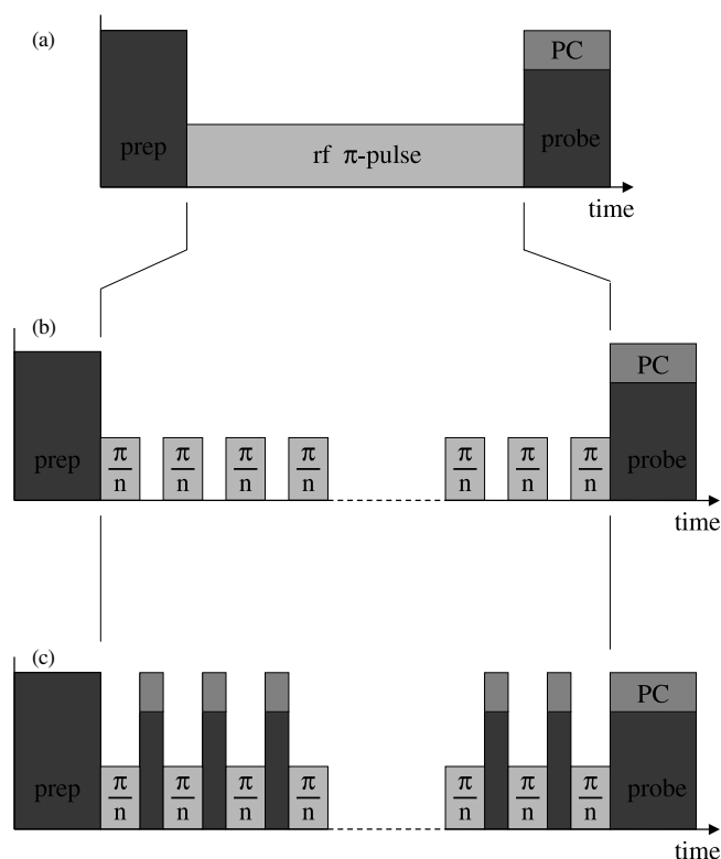
Figure 8. Scheme of measurement with (a) one driving \pi pulse, (b) with fractionated \pi pulse ( n -times \pi/n ), no intermediate probing, and (c) with \pi/n pulses alternating with probe pulses. PC: photon counting.
