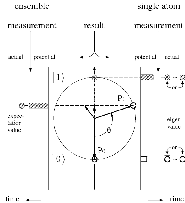
Figure 2. Preparation and measurement of two-level quantum system ( SU(2) ). P_0 initial state vector, P_1 after preparation, by pulse with area \theta , of single quantum system (right). The expectation value from a measurement on an ensemble (left) may result from any P_1 state located at the horizontal plane indicated by the dashed line. Any such mixed state located inside the Bloch sphere would result from phase decoherence by interaction with measuring device, neighbour atoms, or environment. In contrast, a single-atom measurement makes use of a pure state P_1 , located on the surface of the Bloch sphere, that results from the preparation P_0 \rightarrow P_1 . The small bars indicate the probabilities of the results of measurement anticipated from \theta ; they are different, in general, for |0\rangle and |1\rangle . The actual result is an eigenvalue: 1 (and not 0), or 0 (and not 1).
