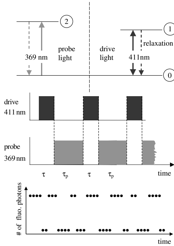
Figure 3. Alternating opto-optical double resonance: scheme of levels and excitation of ^{172}\text{Yb}^+ (top). Temporal schedule (middle). Schematic trajectory of results (bottom).
