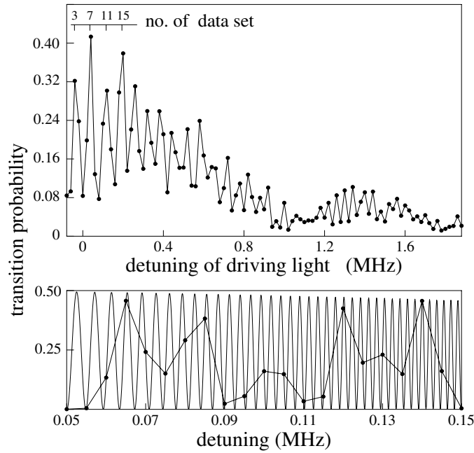
Figure 4. Probability of excitation, versus detuning (\omega - \omega_0)/2\pi by 20 kHz steps of the drive (top). Note the first-order vibronic sideband at 1.3 MHz. Within a small range close to resonance, detuning may replace variation of the drive-pulse length \tau . The spectrum of absorption is superimposed by stroboscopic sampling of the ion's Rabi notation, as demonstrated by a simulation with small steps on an expanded scale (bottom).
