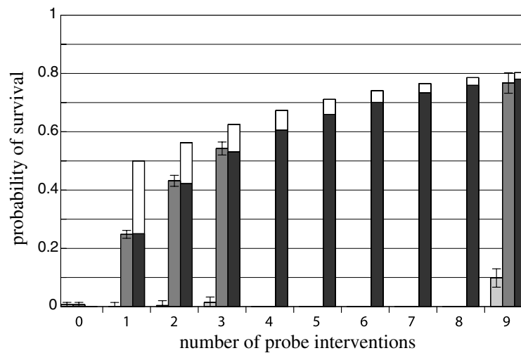
Figure 9. Probability of survival in the ‘off’ state with intermediate probing (dark grey bars), and with no probing (light grey bars), versus number n of \pi -pulse partition. The probability is evaluated by counting as ‘favourable’ those measurements that show only ‘off’ results in each of the n observations. Driving time 2.9 ms, probing time 3 ms. Probability of survival in a ‘selective’ measurement, calculated after equation (4) (black bars). If evaluated from the entire ensemble of results, including intermediate ‘on’ results, such a probability of retrieval would represent a non-selective measurement. This probability is calculated after equation (5) (white bars).
