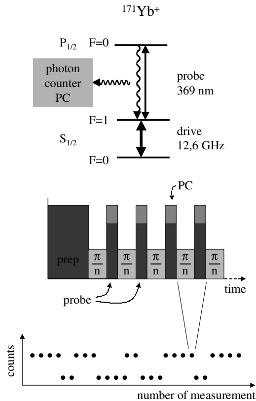
Figure 6. Alternating double resonance on individual ^{171}\text{Yb}^+ ion: scheme of excitation and detection (top), temporal strategy of measurements (middle), trajectory of results (bottom).
