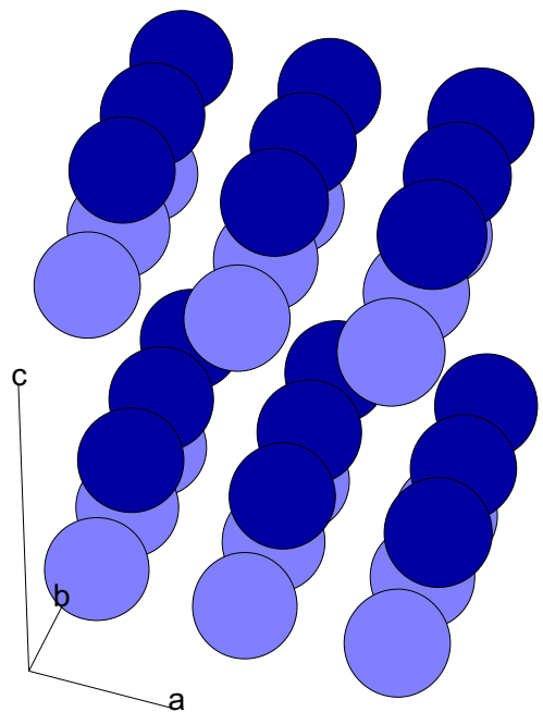
hcp - lattice
