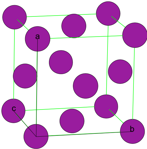
fcc - lattice
